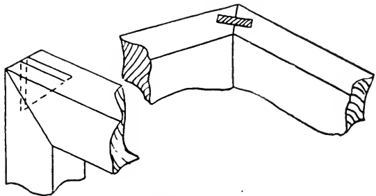
SPLINE MITER
